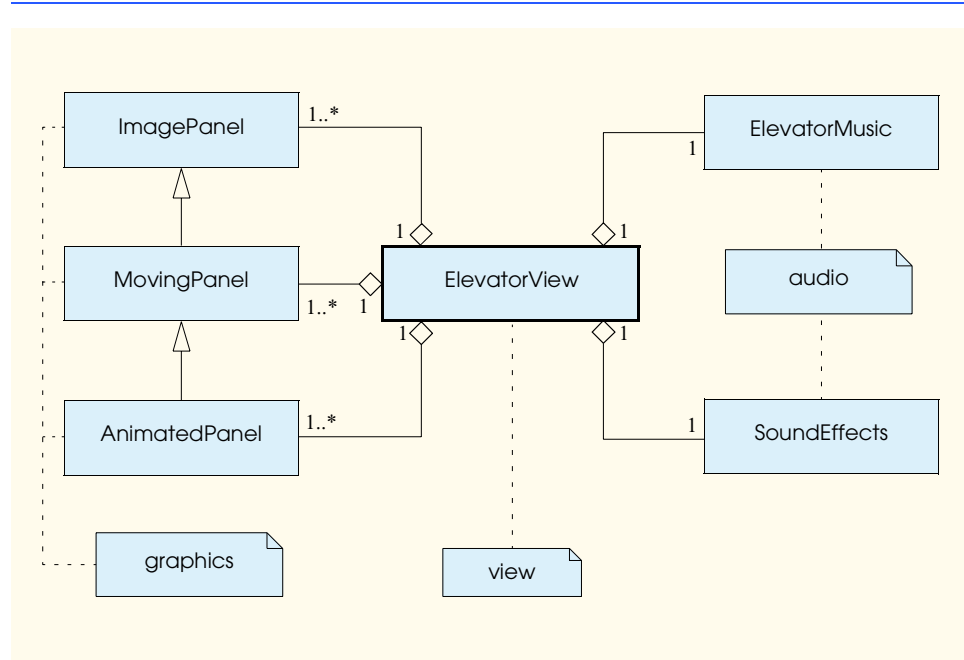
Fig. 22.9 Class diagram of elevator simulation view.
