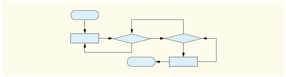
Fig. 5.27 An unstructured flowchart.
