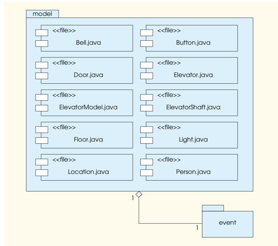
Fig. H.14 Component diagram for package model .
