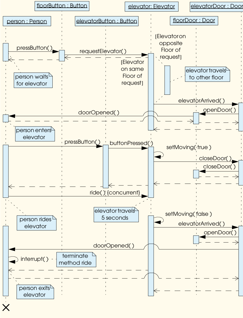
Fig. 15.9 Sequence diagram for a single Person changing floors in system.
