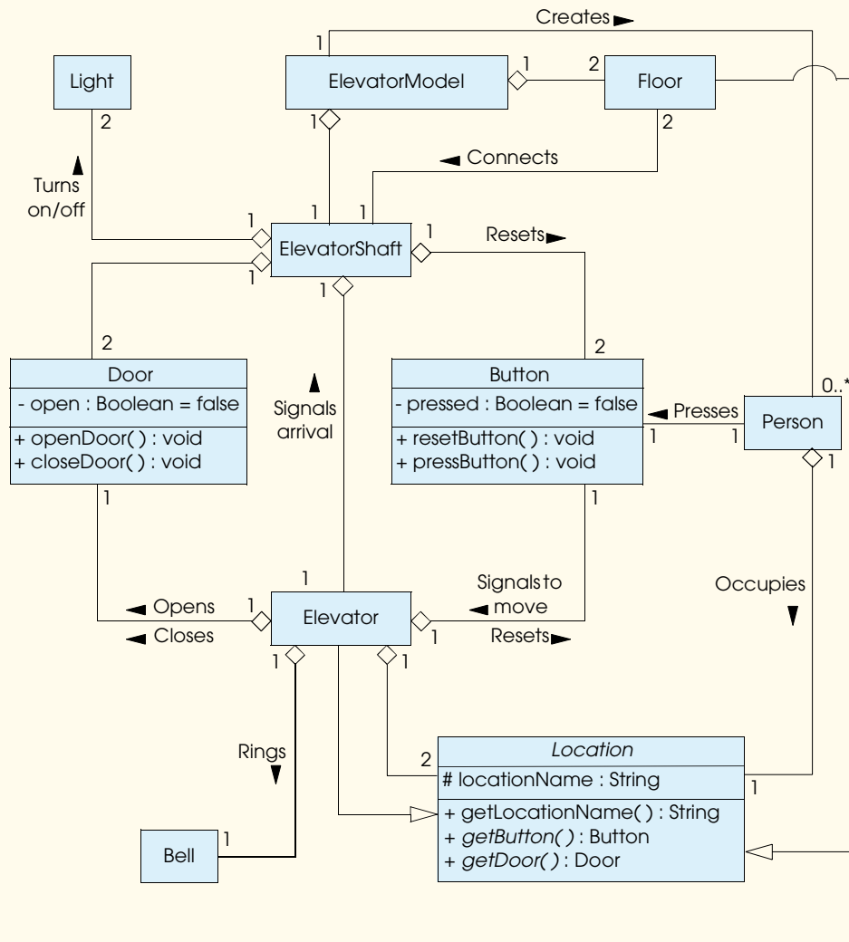
Fig. 9.38 Class diagram of our simulator (incorporating inheritance).
