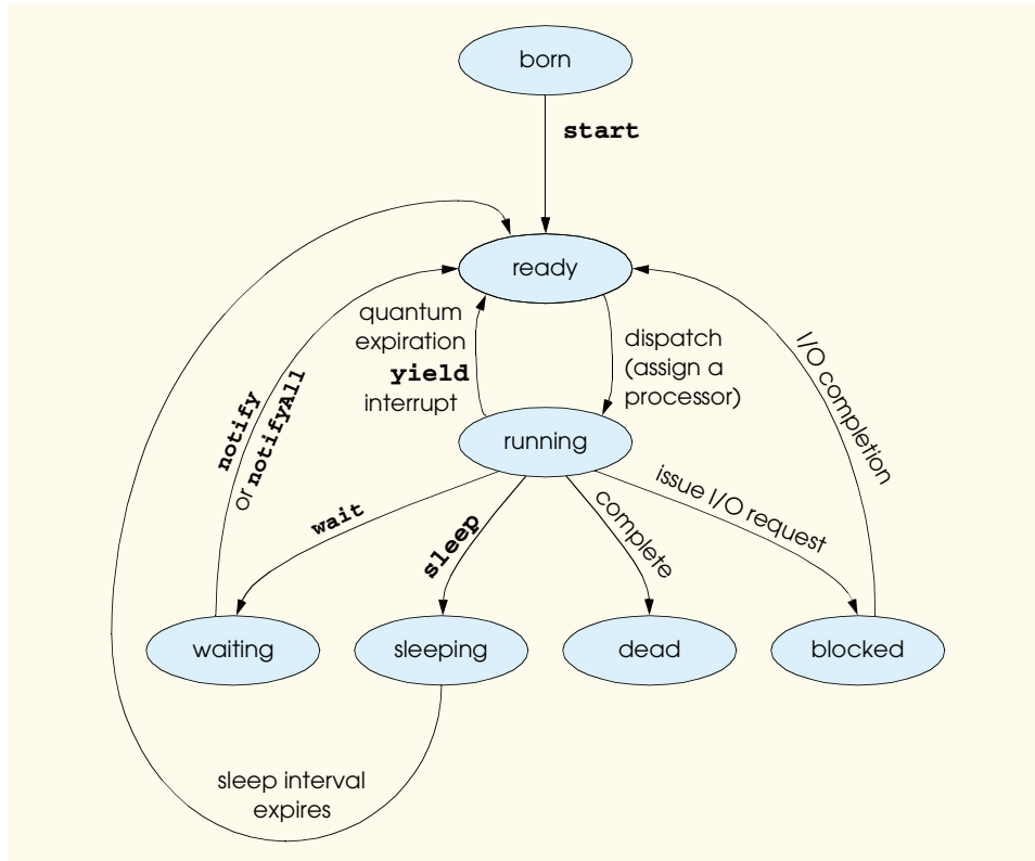
Fig. 15.1 State diagram showing the Life cycle of a thread.
