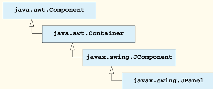
Fig. 13.22 Inheritance hierarchy for class JPanel .
