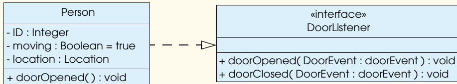
Fig. 11.24 Class diagram that models class Person realizing interface DoorListener .
