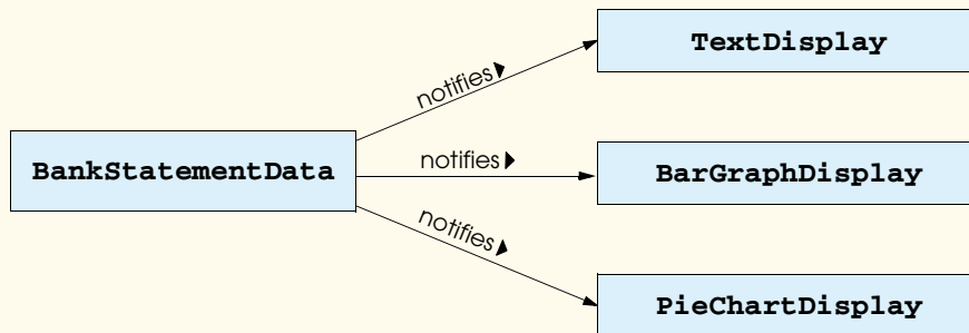
Fig. 13.23 Basis for the Observer design pattern.
