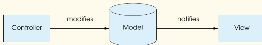
Fig. 17.22 Model-View-Controller Architecture.
