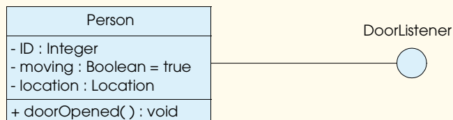
Fig. 11.25 Elided class diagram that models class Person realizing interface DoorListener .
