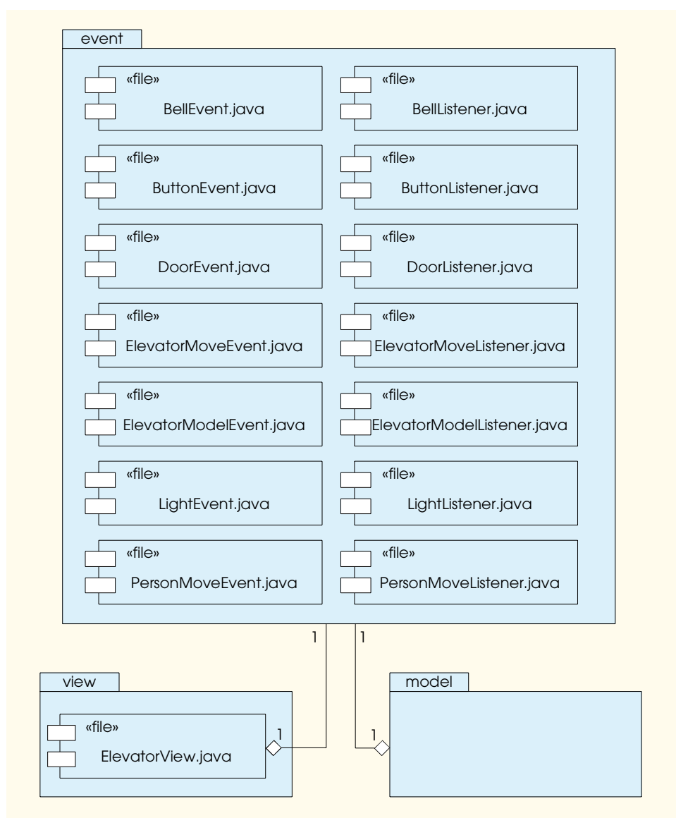
Fig. G.15 Component diagram for package event .
